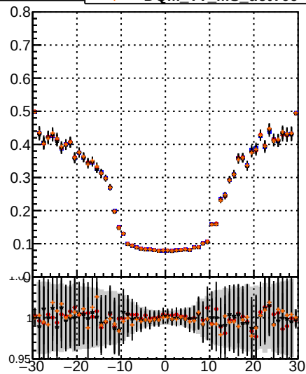
Fake rate vs v_z Line Style Color Symbol Model Detector Solid Blue Circle DOM TT Solid Red Circle DOM MS Dashed Blue Circle DOM detT Dashed Red Circle DOM detT1 Dashed Blue Circle DOM detT09 Dashed Red Circle DOM detT09
