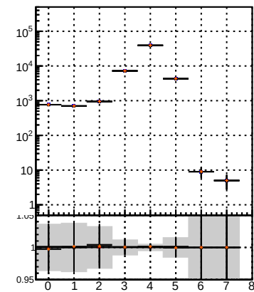
N of simulated tracks vs pixel layer
