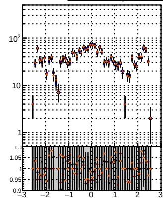
N of reco track vs \eta Legend: BQM (blue), TT (red), MS (green), delT (orange), delTb9 (purple)
