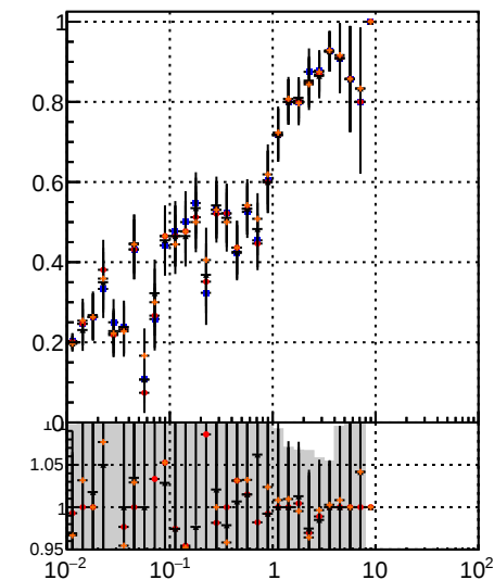
Fake rate vs \sqrt{s} Legend: BQM TT MS detT (blue) BQM TT MS detT1 (red) BQM TT MS detT09 (orange) BQM TT MS detT109 (grey)
