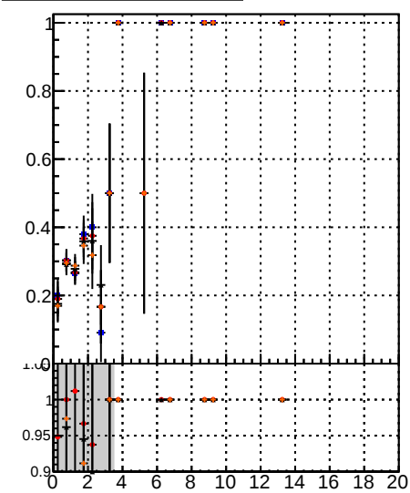
Fake rate vs. BSM MS det1 BSM MS det109
