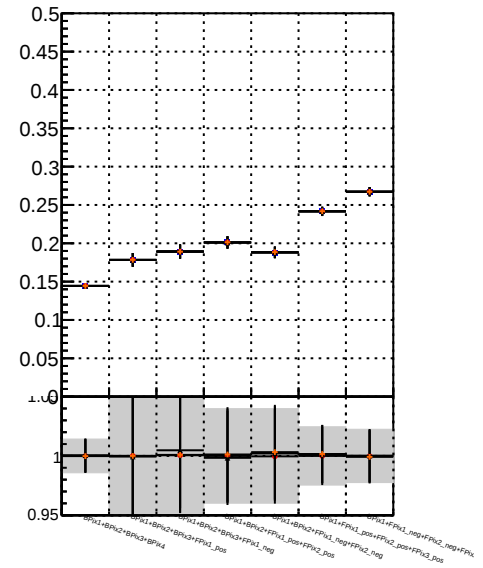
Fake rate vs. DSM IT MS det1 DSM IT MS det109
