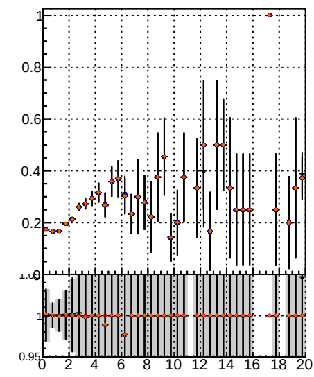
Fake rate vs. DSM IT MS det1 DSM IT MS det109
