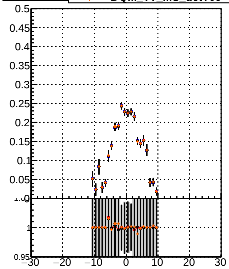
Fake rate vs \sqrt{s} Legend: DOM TT MS detT DOM TT MS detT1 DOM TT MS detT09
