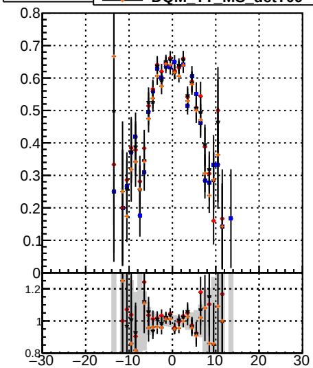
Fake rate vs v_{\text{rel}} Category Color Shape \text{BQM} \rightarrow \text{TT} Blue Square \text{BQM} \rightarrow \text{MS} Red Triangle \text{BQM} \rightarrow \text{detT} Orange Circle \text{BQM} \rightarrow \text{detT1} Grey Star
