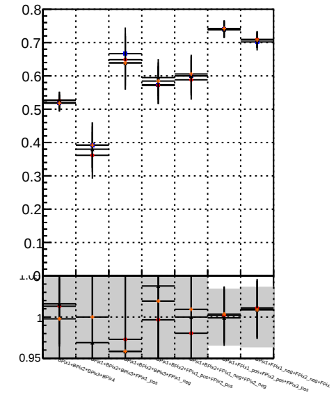
Fake rate vs. \text{BSM} \parallel \text{MS det1} \text{BSM} \parallel \text{MS det109}
