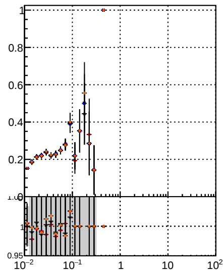
Fake rate vs v DOM TT MS detT DOM TT MS detL1 DOM TT MS detL09
