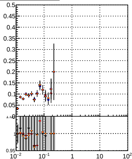
Fake rate vs v Legend: DOM TT MS detT, DOM TT MS detL1, DOM TT MS detL09
