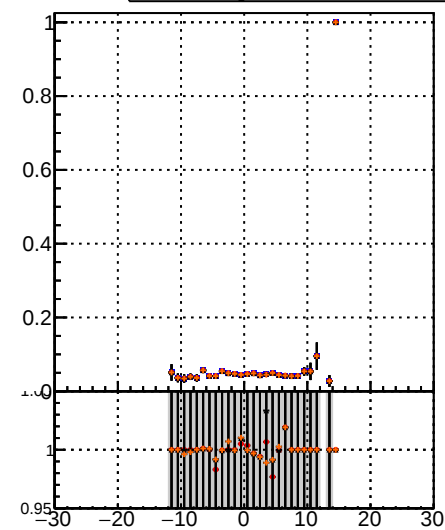
Fake rate vs v Legend: DOM TT MS detT, DOM TT MS detL1, DOM TT MS detL09
