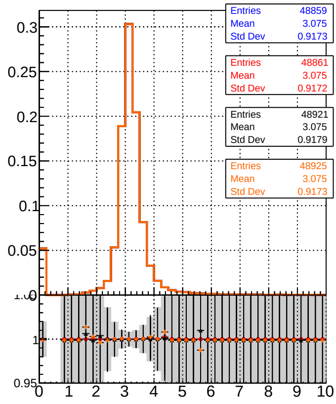
Legend: DQM_TT_MS (blue line), DQM_TT_MS_detT (red line with dots), DQM_TT_MS-detT1 (black line with dots), DQM_TT_MS_detT09 (orange line with dots)
