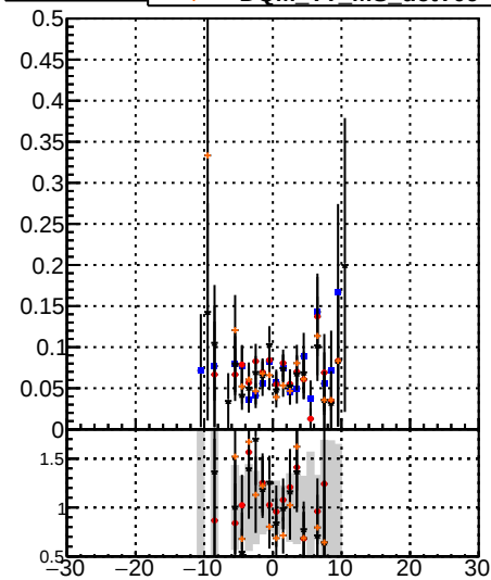
Fake rate vs v Legend: DOM TT MS detT DOM TT MS detT1 DOM TT MS detT09
