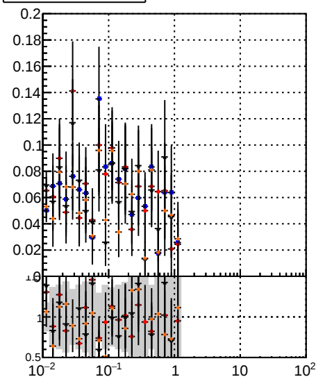
Fake rate vs v Legend: DOM TT MS detT DOM TT MS detT1 DOM TT MS detT09
