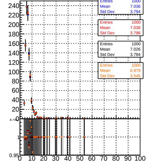
Uncertainty x Coordinate (other Vtx)
