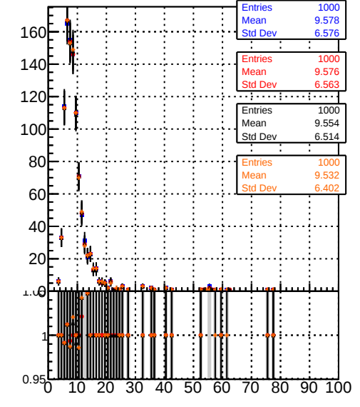
Uncertainty z Coordinate (tagged Vtx)
