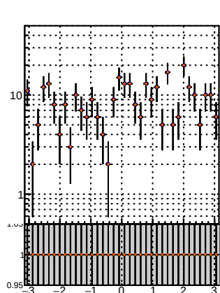
N of associated (recoToSim) duplicate tracks vs phi
