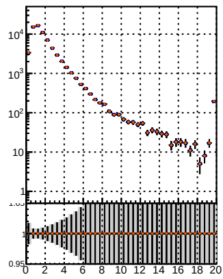
N of associated (recoToSim) tracks vs. \chi^2
