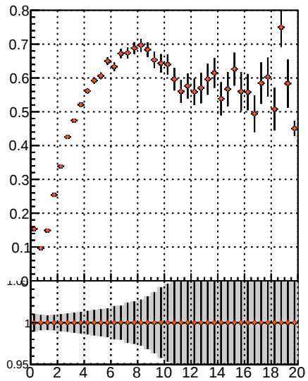
Fake rate vs. BQM MS det1 BQM MS det09
