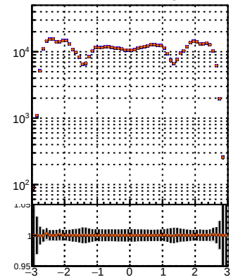
N of reco track vs \eta Legend: BQM (black), TT (red), MS (blue), delT (orange)
