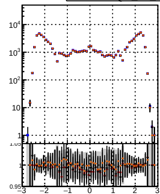
N of reco track vs \eta Legend: BQM (black), TT (red), MS (blue), detT (orange)
