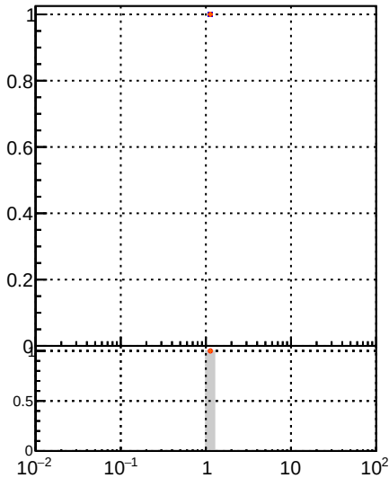
Fake rate vs v_z
