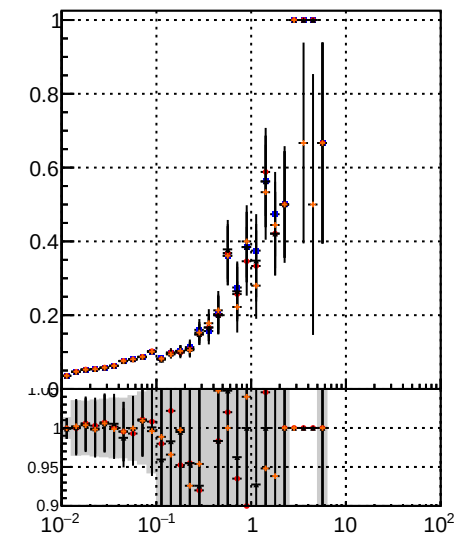
Fake rate vs v_z Legend: DOM TT MS detT DOM TT MS detT1 DOM TT MS detT09
