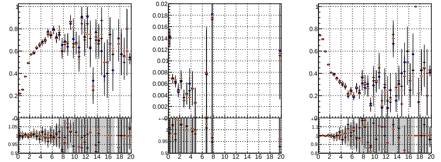
Fake rate vs. \chi^2
