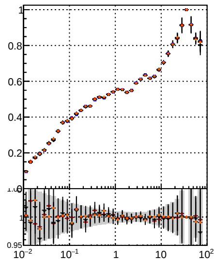
Fake rate vs \nu BQM TT MS detT BQM TT MS detT1 BQM TT MS detT09 BQM TT MS detT109
