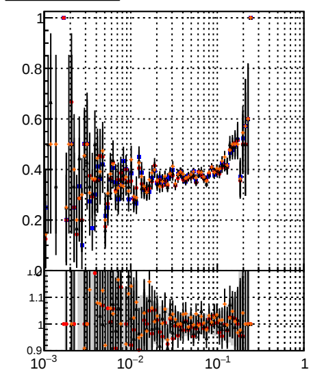
Pileup rate vs \mu
