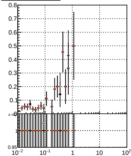
Fake rate vs \nu — DOM TT MS detT — DOM TT MS detT1 — DOM TT MS detT09
