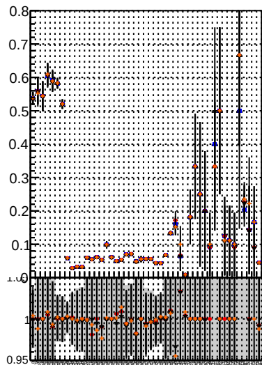
Fake rate vs. BSM MS det109 BSM MS det109
