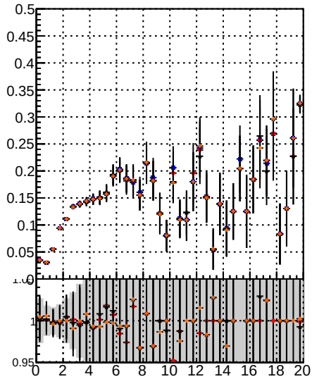
Fake rate vs. BSM MS det109 BSM MS det109
