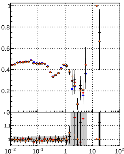
Fake rate vs \nu Legend: DQM TT MS detT (blue squares) DQM TT MS detT1 (orange circles) DQM TT MS detT09 (red triangles) MS detT (black crosses)
