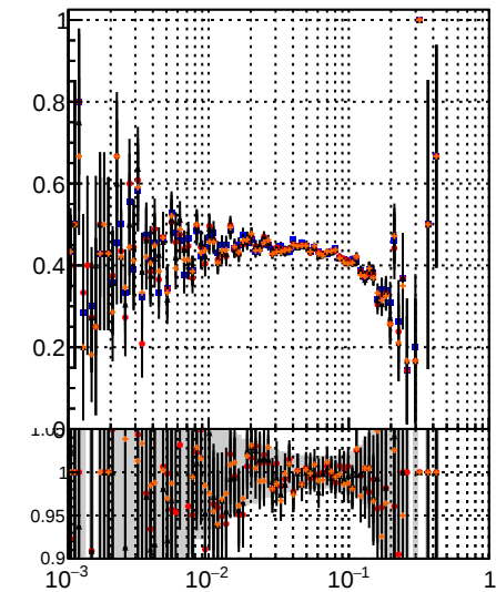
Fake rate vs \sqrt{s} Category Color Shape BQM TT MS detT Blue Square BQM TT MS detT1 Red Circle BQM TT MS detT09 Orange Triangle BQM TT MS detT109 Black Cross
