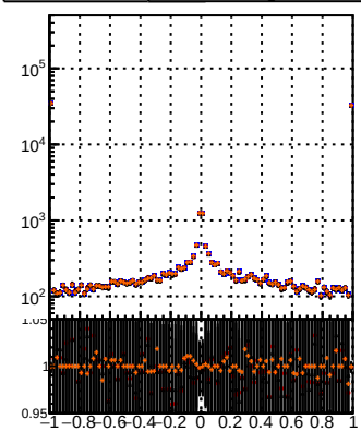
Legend for track types: DOM (black) TT (red) MS (blue) detT (green) detT-dpda (orange)
