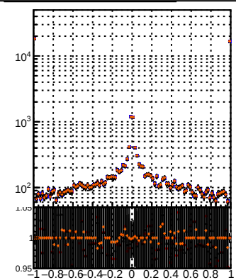
Legend for track types: DOM (black) TT (red) MS (blue) detT (green) detT-dpda (orange)
