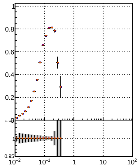
Fake rate vs v Legend: \text{BQM} (blue line), \text{TT} (red line), \text{MS} (black line), \text{detT} (orange line), \text{dpdq} (green line), \text{detT-chi2} (purple line)
