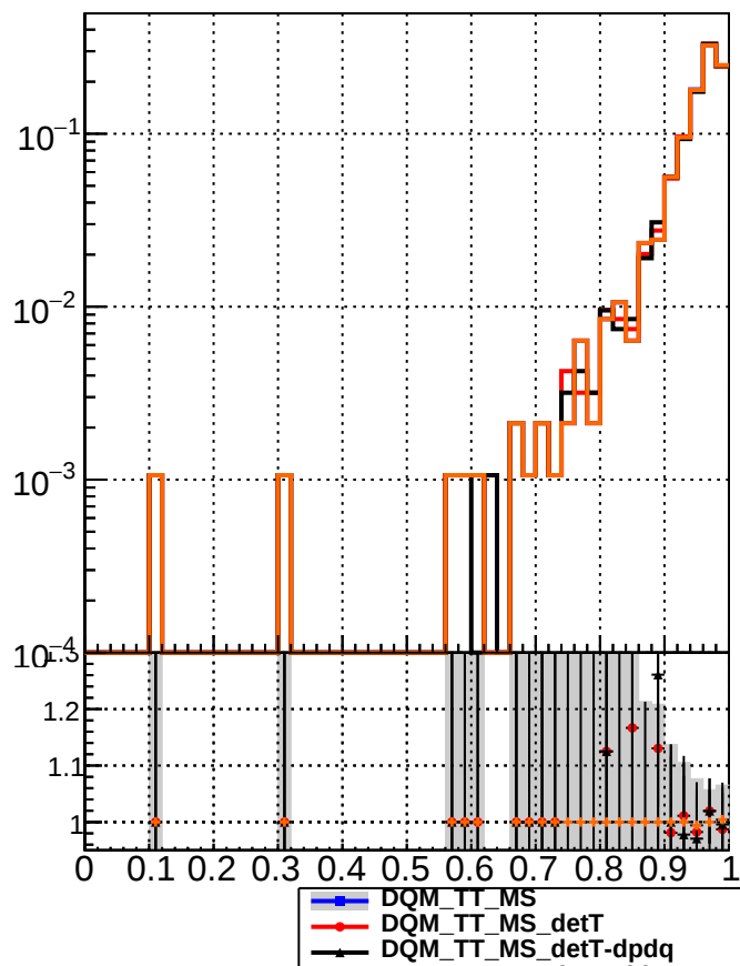
RecoPVAssoc2GenPVMatched_missing
