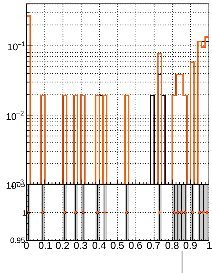
RecoPVAssoc2GenPVNotMatched_missing
