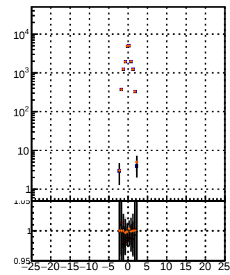
Legend for track types: TT (black line) MS (red line) defT (blue line) defT-dpda (orange line) defT-chi2 (green line)
