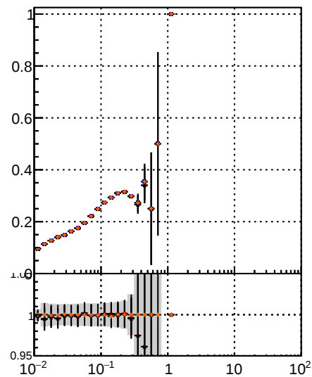
Fake rate vs \sqrt{s} Legend DOM TT MS detT dpdg detT-chi2 Line Blue Red Green Black Orange Grey Point Blue Red Green Black Orange Grey
