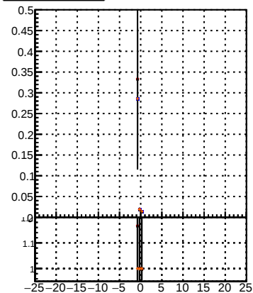
Fake rate vs d Legend: DOM TT MS DOM TT MS detT DOM TT MS detT-dpdq DOM TT MS detT-chi2
