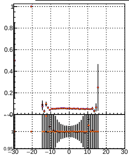
Fake rate vs v DOM TT MS detT DOM TT MS detT-dpdaq DOM TT MS detT-chi2
