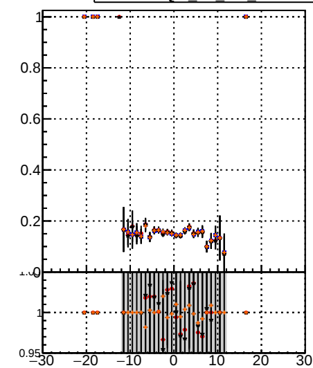
Fake rate vs \sqrt{s} BQM TT MS detT BQM TT MS detT dndq BQM TT MS detT chi2
