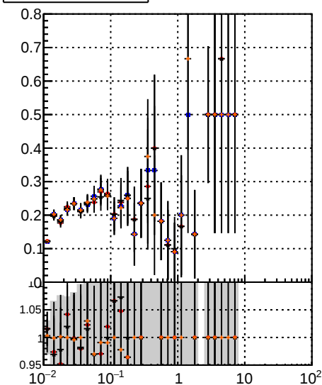
Fake rate vs \sqrt{s} BQM TT MS detT BQM TT MS detT dndq BQM TT MS detT chi2
