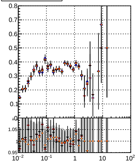
Fake rate vs \sqrt{s} BQM TT MS detT BQM TT MS detT-dpdq BQM TT MS detT-chi2
