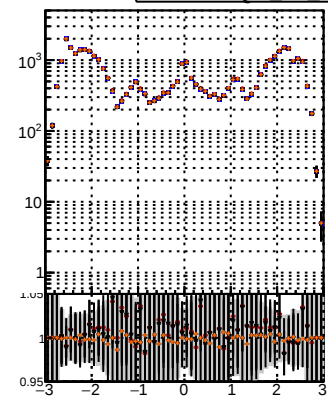
N of reco track vs \eta BQM TT MS delT-delta2 BQM TT MS delT-delta2 BQM TT MS delT-delta2 BQM TT MS delT-delta2
