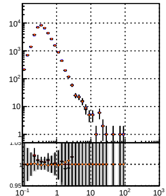
N of reco track vs \eta BQM TT MS delT-delta2 BQM TT MS delT-delta2 BQM TT MS delT-delta2 BQM TT MS delT-delta2
