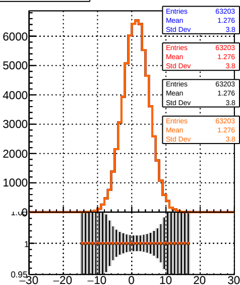
GeneratedAIV_Z
