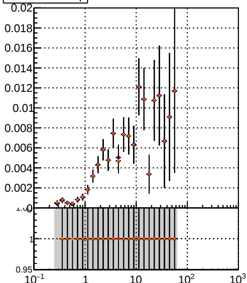
Efficiency vs p_T
