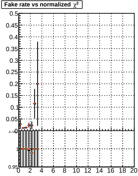
Fake rate vs. Model Normalized \chi^2 Fake Rate BOM 0.5 0.02 TT 2.0 0.12 MS 2.0 0.02 data 2.0 0.02
