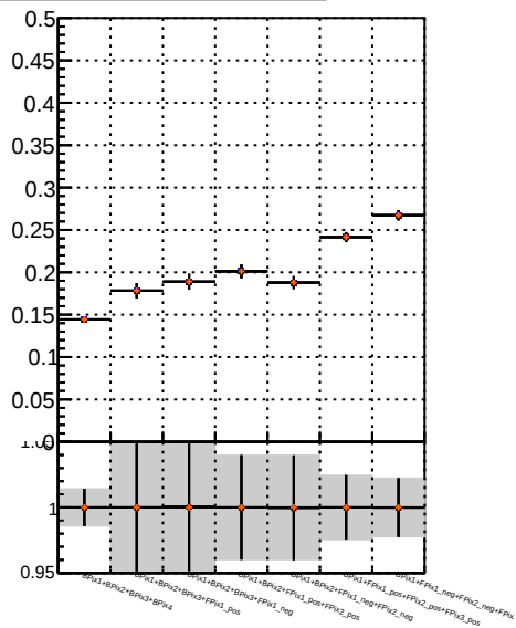
Fake rate vs. BGM TT MS detT detT-dpdq detT-chi2
