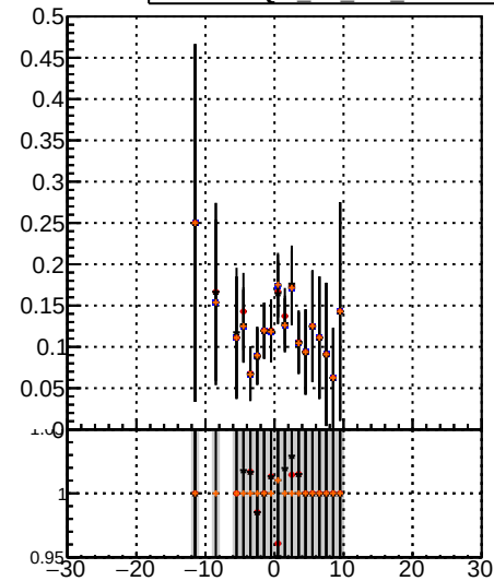
Legend: - \text{BQM TT MS detT dpgq} - \text{BQM TT MS detT chi2}
