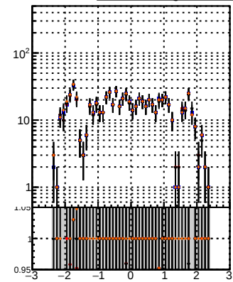
N of reco track vs \eta BQM TT MS delT delT-delta2 BQM TT MS delT delT-delta2
