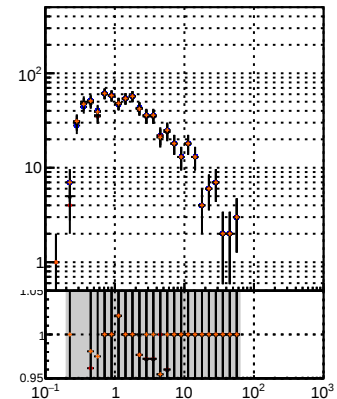
N of reco track vs \eta BQM TT MS delT delT-delta2 BQM TT MS delT delT-delta2
