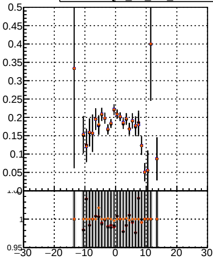
Fake rate vs v BQM TT MS detT dpg detT-chi2 BQM TT MS detT dpg detT-chi2
