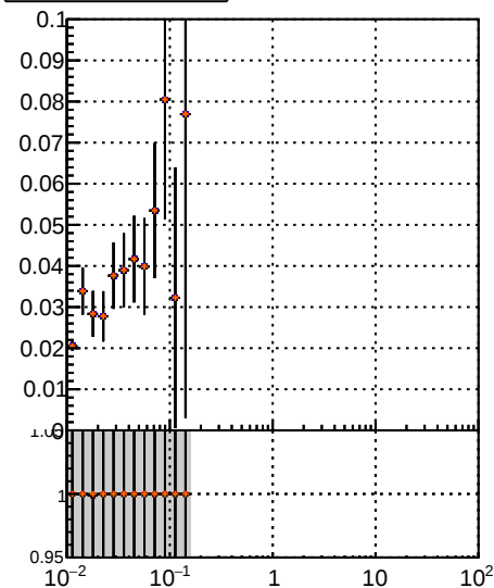
Fake rate vs \sqrt{s} —●— \text{BQM TT MS detT} —●— \text{BQM TT MS detT-dpdq} —●— \text{BQM TT MS detT-chi2}
