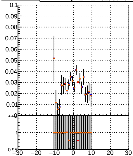
Fake rate vs v Legend: B0M \rightarrow TT \rightarrow MS detT, B0M \rightarrow TT \rightarrow MS detT-dpdp, B0M \rightarrow TT \rightarrow MS detT-chi2
