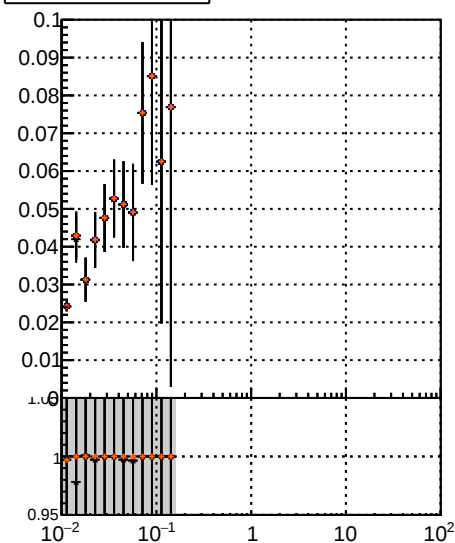
Fake rate vs v Legend: B0M \rightarrow TT \rightarrow MS detT, B0M \rightarrow TT \rightarrow MS detT-dpdp, B0M \rightarrow TT \rightarrow MS detT-chi2
