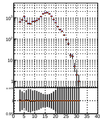
BQM TT MS defT-dpda BQM TT MS defT-chi2 N of reco track vs hit
