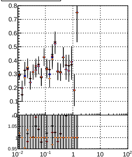
Fake rate vs v Legend Color Shape Line Style BQM Blue Circle Solid TT Red Circle Solid MS Black Circle Solid detT Black Circle Solid dpgq Black Circle Solid detT-chi2 Black Circle Solid
