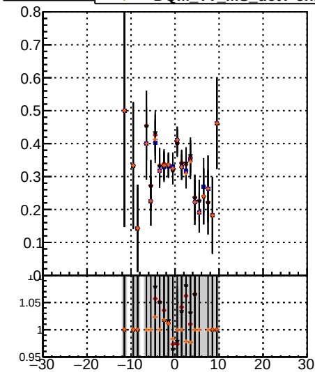
Fake rate vs v Legend Color Shape Line Style BQM Blue Circle Solid TT Red Circle Solid MS Black Circle Solid detT Black Circle Solid dpgq Black Circle Solid detT-chi2 Black Circle Solid
