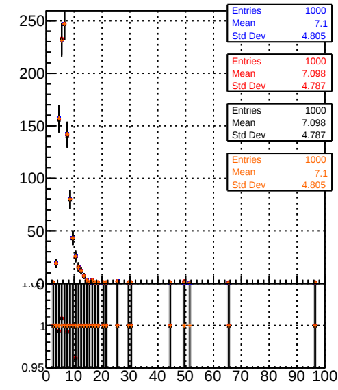
Uncertainty x Coordinate (other Vtx) (tagged Vtx)
