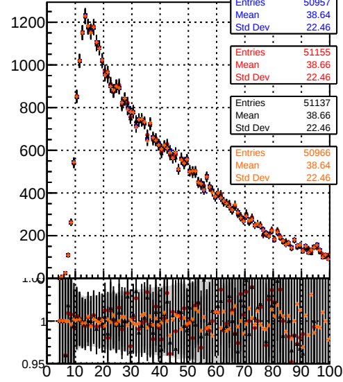
Uncertainty x Coordinate (other Vtx) (tagged Vtx)
