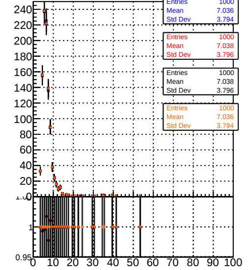
Uncertainty x Coordinate (other Vtx) (tagged Vtx)
